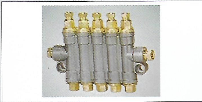
METERING CARTRIDGE HBL
